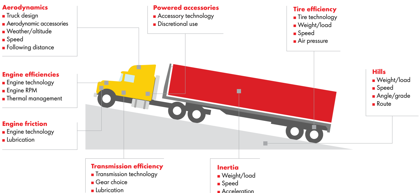
FIGURE 2. Factors influencing the fuel economy of a tractor-trailer truck setup.
